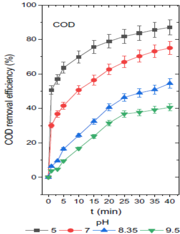
Figure 3. Variations in COD concentration and removal efficiencies of leachate at different pH values in the electrocoagulation process.
