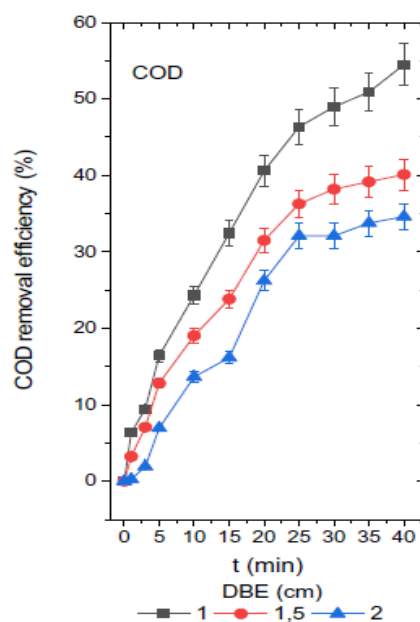
Figure 5. Variations in COD concentration and removal efficiencies of leachate at different inter-electrode distance values in the electrocoagulation process.
