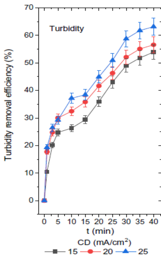
Figure 2. Changes in the concentration of turbidity and the efficiency of leachate removal at various levels of current density in the electrocoagulation process.
