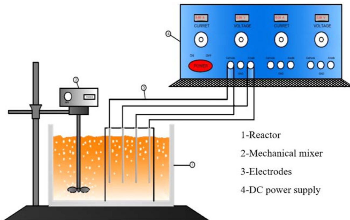
Figure 1. Electrocoagulation process
