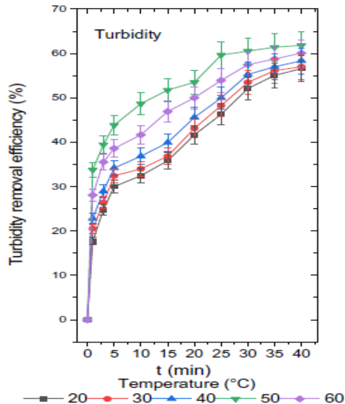
Figure 4. Changes in the concentration of turbidity and the efficiency of leachate removal at various levels of temperatures in the electrocoagulation process.
