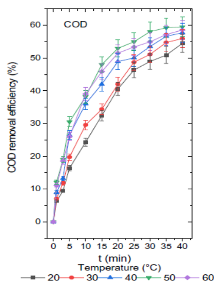
Figure 4. Variations in COD concentration and removal efficiencies of leachate at different temperature values in the electrocoagulation process.
