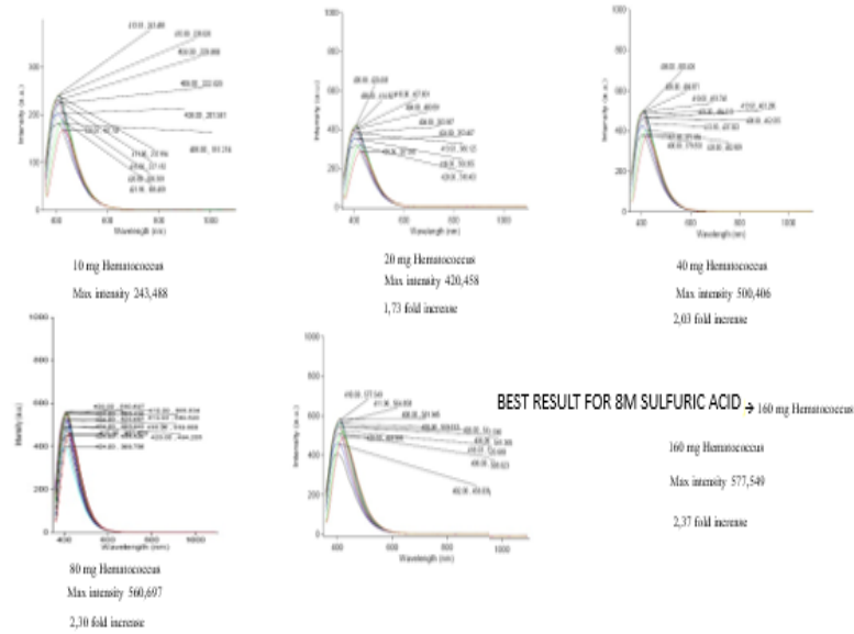
Figure 5. Microwave Experiment's Results with Sulfuric acid
