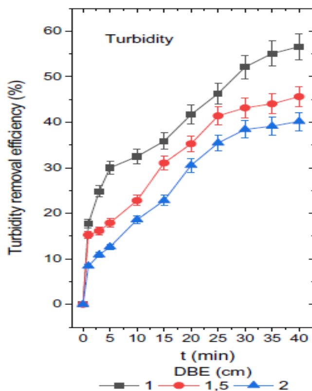
Figure 5. Changes in the concentration of turbidity and the efficiency of leachate removal at various levels of inter-electrode distance in the electrocoagulation process.
