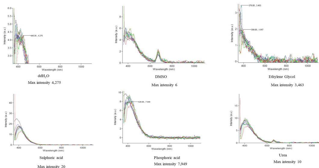
Figure 2. Microwave Experiment's Results
