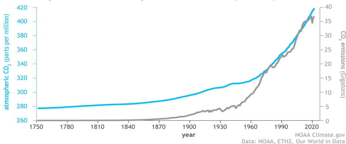
Figure 1. Global atmospheric carbon dioxide compares to annual emissions (1751-2022) (Anonymous, 2024)
