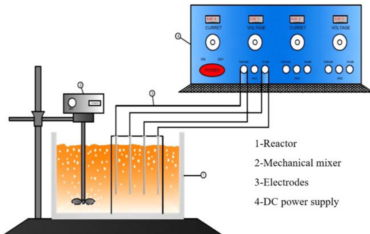
Figure 1. Electrocoagulation process
