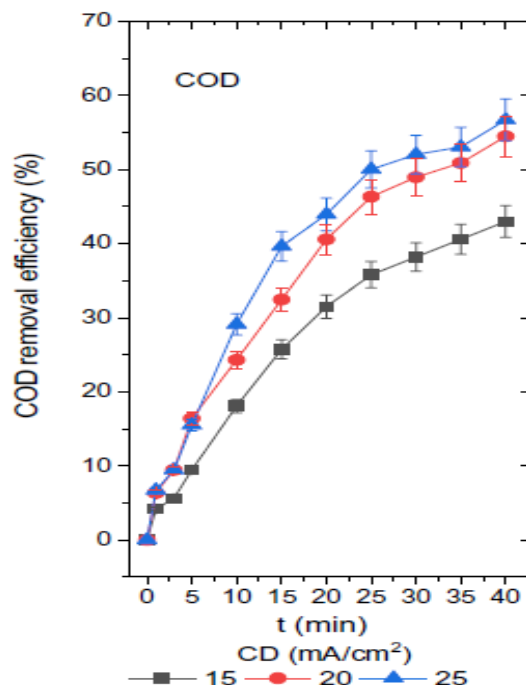
Figure 2. Variations in COD concentration and removal efficiencies of leachate at different current density values in the electrocoagulation process.
