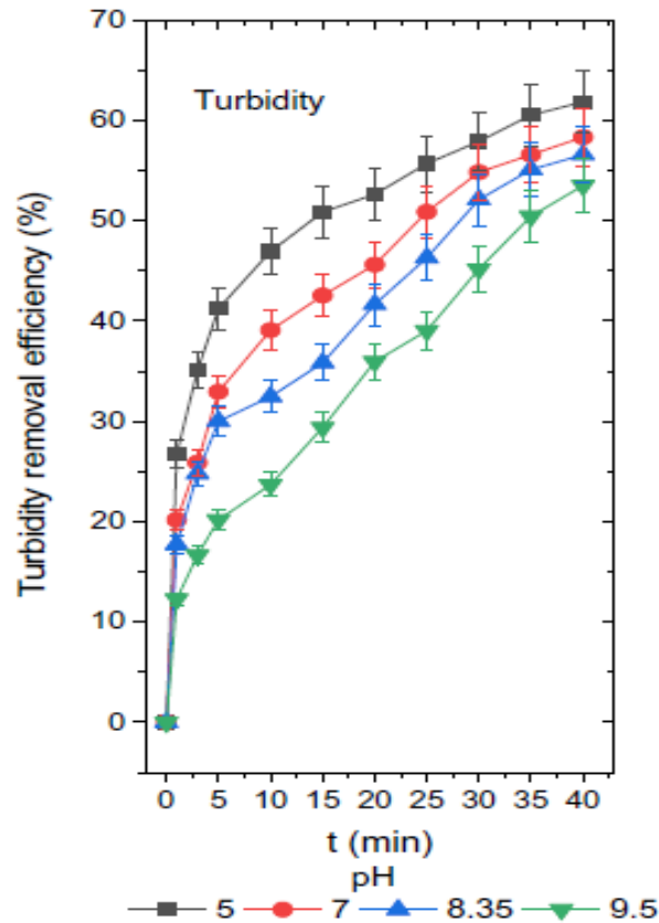
Figure 3. Changes in the concentration of turbidity and the efficiency of leachate removal at various levels of pH in the electrocoagulation process.
